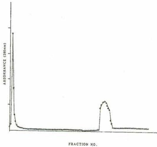
Fig 2. Ion exchange chromatography on Amberlite IRC-120.
