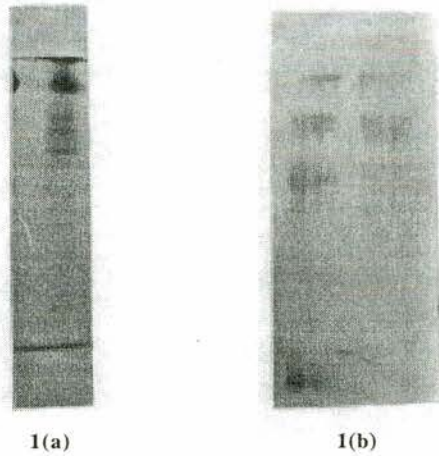
Fig 1(a). Electrophoresis of crude extract. Fig 1(b). Electrophoresis of fractions of Amberlite IRC-120.
