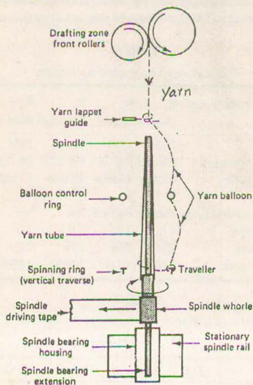
Fig 1. Ring spinning frame (side elevation/section).
